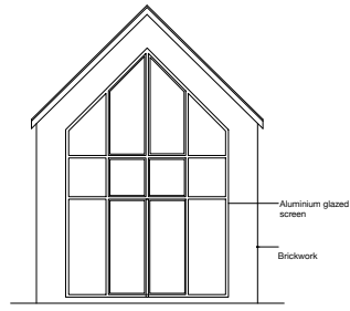
North West Elevation
